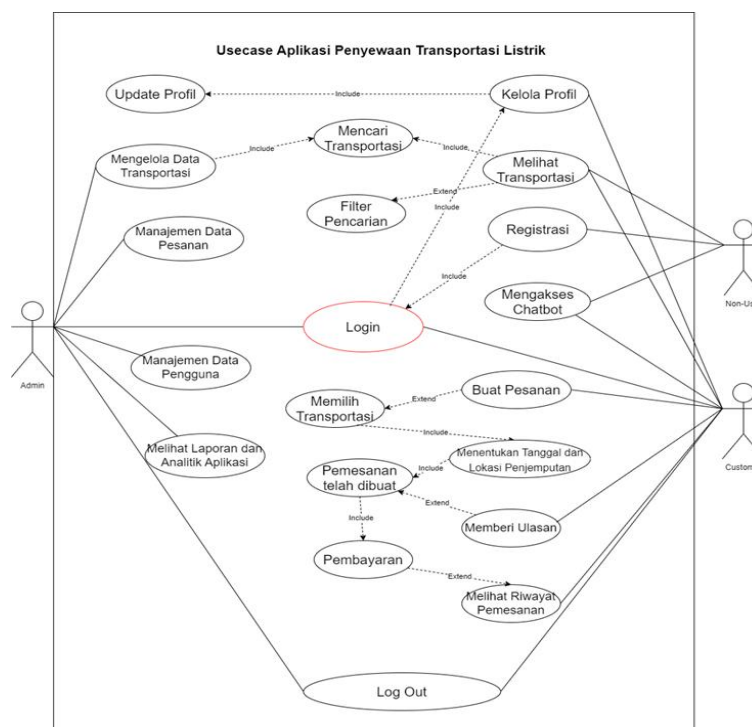
Gambar 3. Usecase Diagram
